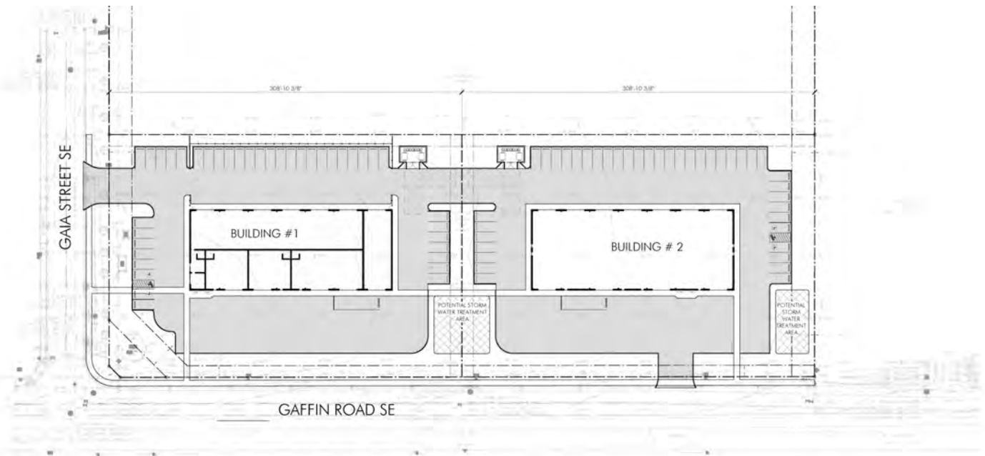
Preliminary Site Plan of Subject Property
